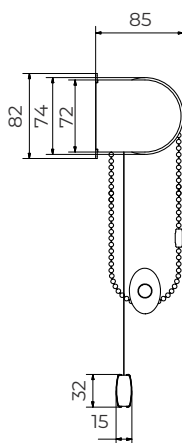
40+® standard metal bracket face fix & cover
