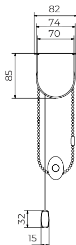
40+® standard metal bracket top fix & cover
