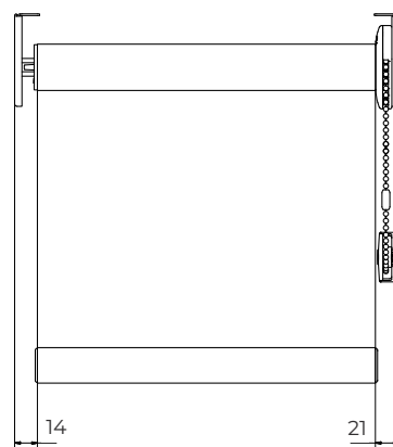
40+® standard metal bracket top fix front view
